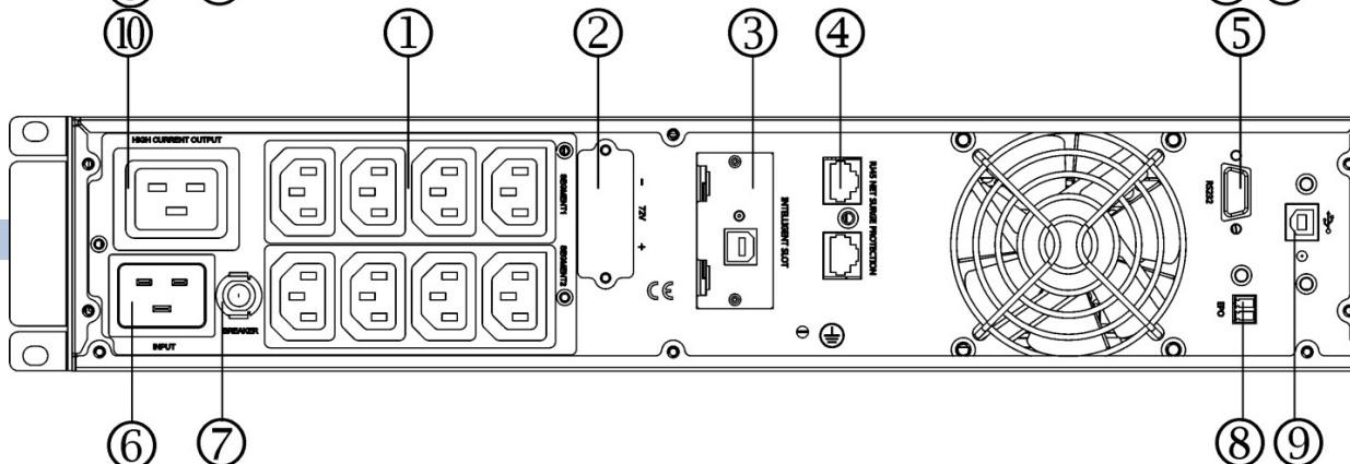
M9103S-RT 3kVA
