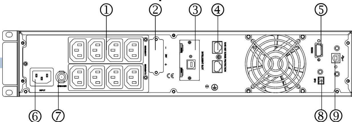
M9101S-RT 1kVA
