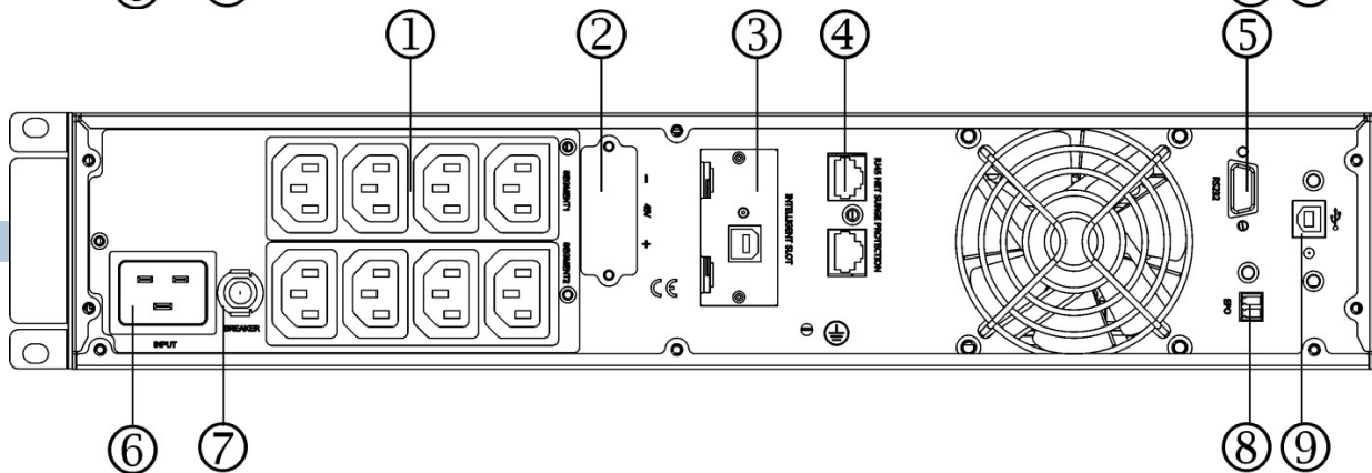
M9102S-RT 2kVA
